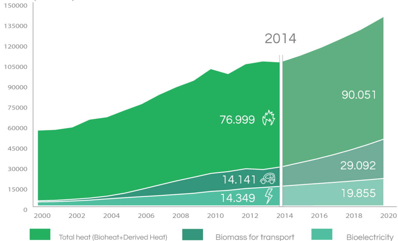
Gross final energy consumption of bioenergy 2000-2014 (in ktoe)
